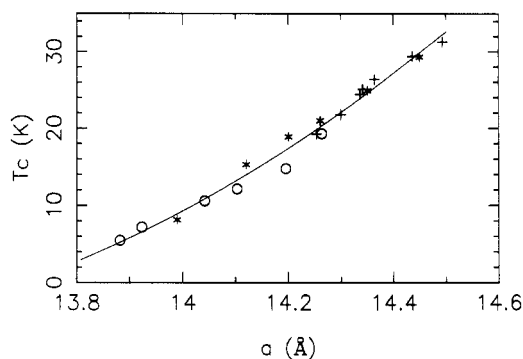
Figure 5. Superconducting transition temperature versus lattice parameter. a(P) X-ray data converted to T_c(a) using the raw T_c(P) data of Sparrn. 49 (O) K_3C_{60} ; (*) Rb_3C_{60} ; + symbols are the directly-measured points from a number of M_{3-x}M'_x C_{60} compounds at 300 K, 1 bar. 48 The solid curve is a quadratic fit. 50
